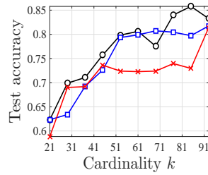
(g) Log. synthetic ( \tau = 20 )
