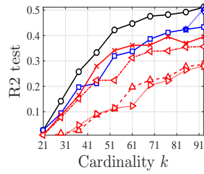
(c) Lin. reg. ( \tau = 20 )
