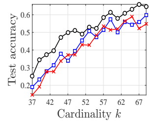
(l) MNIST ( \tau = 35 )
