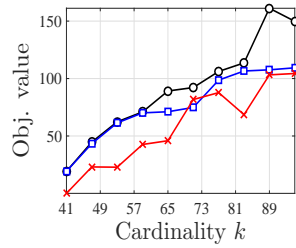
(f) Log. synthetic ( \tau = 40 )
